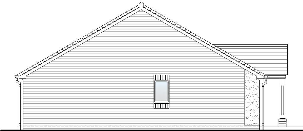
Left Elevation
