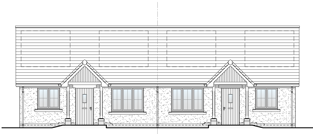
Front Elevation
